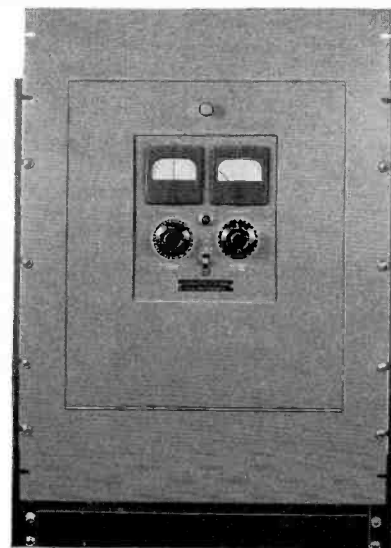
The operating console for the 50-kw transmitter provides single push-button starting for the entire transmitter with automatic sequence. Controls and indicator devices are provided for all major operating functions.
